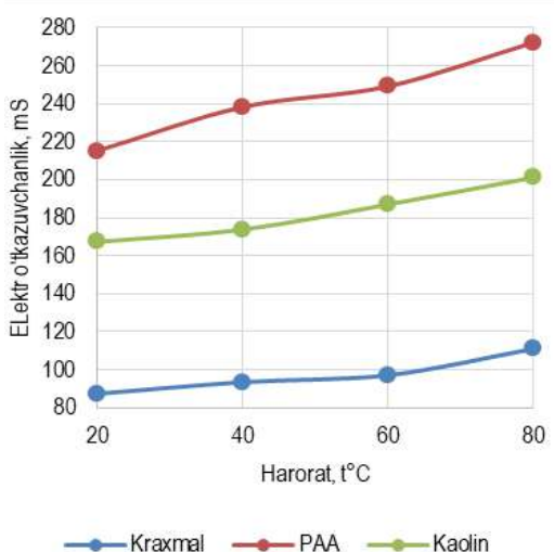
10-rasm. 2g/l NB+50mg/l PAA, kraxmal, kaolin suspenziyalari elektr o'tkazuvchanligi
