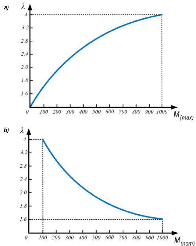
2-rasm. Motorning o'ta yuklama qiymati uning maksimal momentiga proporsionalligi: a - yuklanish koeffitsientini maksimal momentga bog'liqligi; b - yuklanish koeffitsientini nominal momentga bog'liqligi
