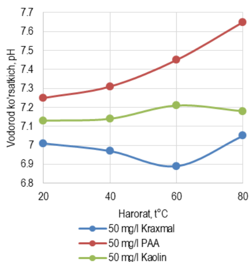
7-rasm. 50 mg/l (kraxmal, PAA, kaolin) suspenziyani turli haroratlardagi pH o'zgarishi
