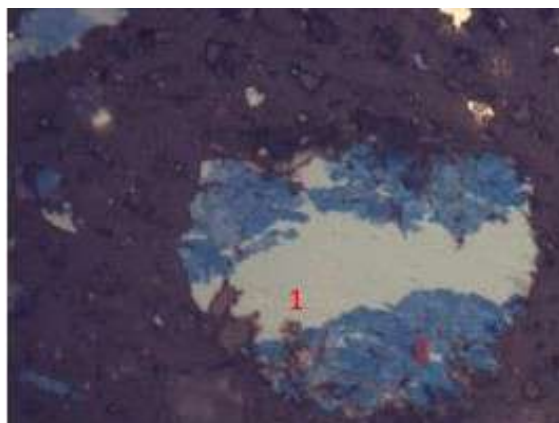
5-rasm. Xalkozin (1) kovellin (2). Kattalashtirilgan 200x
