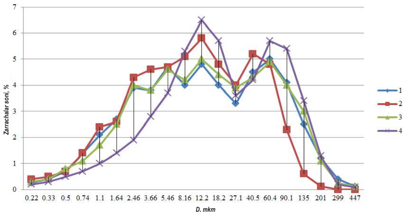
5-rasm. Tegirmonning n = 22 ayl/min tezligida olingan tayyor mahsulotdagi zarrachalar hajmini taqsimlash grafigi va sharlarning turli og'irlikdagi o'rtacha diametri: 1) d_{sh} = 40 mm; 2) d_{sh} = 50 m; 3) d_{sh} = 60 m; 4) d_{sh} = 68 mm
