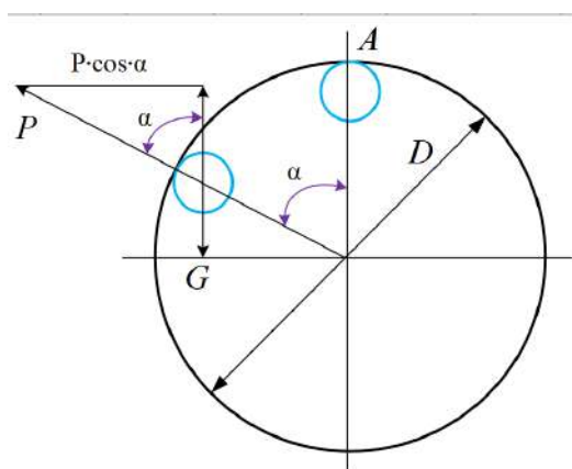
2-rasm. Sharli tegirmon barabanidagi bitta shar yanchish harakatini diagrammasi
