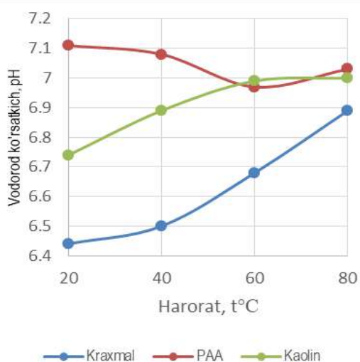
9-rasm. 2g/l NB+50mg/l PAA, kraxmal, kaolin suspenziyalari pH
