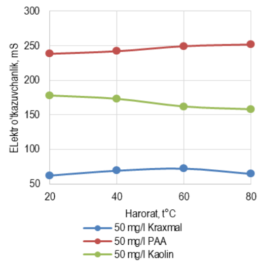
8-rasm. 50 mg/l (PAA, kraxmal, kaolin) suspenziyani turli haroratlardagi elektr o'tkazuvchanligining o'zgarishi
