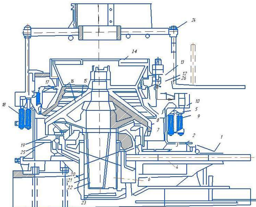
2-rasm. KSD tipidagi konusli maydalagich: 1 – harakatlanuvchi korpus; 2 – stanina; 3 – harakatlanuvchi korpusining qoplamasi; 4 – bloklash tizimi; 5 – prujina tayanchi, 6 – eksentrik chashka; 7 – harakatlanuvchi tayanch qismi; 8 – gidravlik ustun; 9 – prujinali amortizator; 10 – tayanch halqa; 11 – eksentrik val; 12 – stakan; 13 – himoya korpusi; 14 – tayanch halqasi; 15 – harakatlanuvchi konusning qoplamasi; 16 – silindrsimon vtulka; 17 – qo'zg'almas konusning zirhi (futerovkasi); 18 – prujinali amortizator; 19 – aylanish mexanizmi; 20 – silindrsimon vtulka; 21 – konusning qoplamasi; 22 – tayanch halqa; 23 – eksentrik val; 24 – yuklash platformasi; 25 – eksentrik qurilma; 26 – tayanch blok
