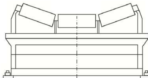
1-rasm. Konveyer rolik tayanchi
