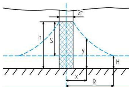
1-rasm. Yuboruvchi quduqdagi depression voronka
